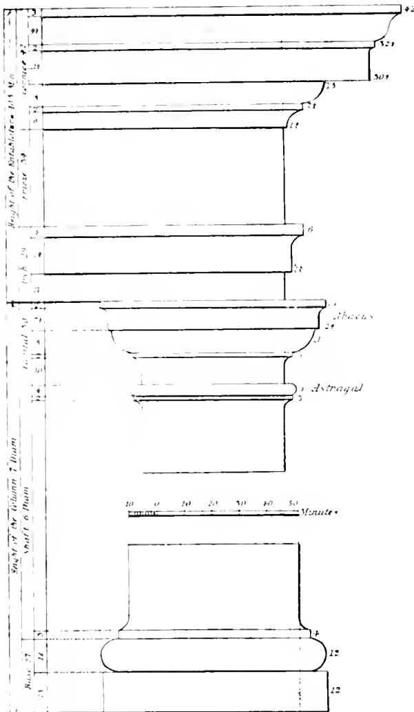
NO. 217.—THE TUSCAN COLUMN AND ENTABLATURE.
